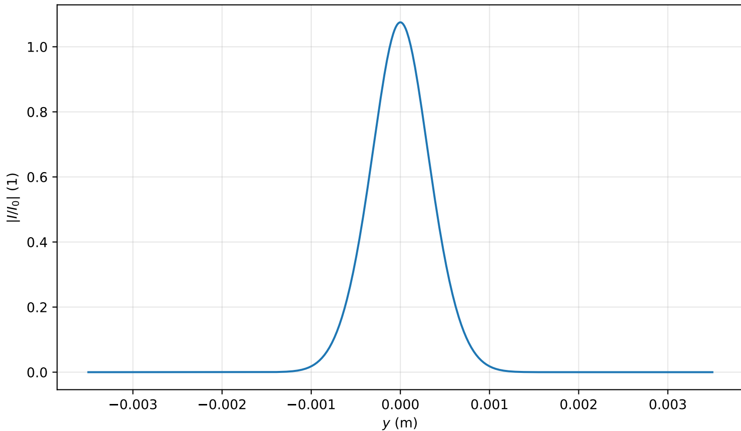
Intensity profile I(x = 0, y, z = 0.318)/I_0 , P_{in}=1.0P_{cr} , artificial time
